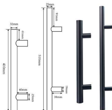
Glass Door Handle
