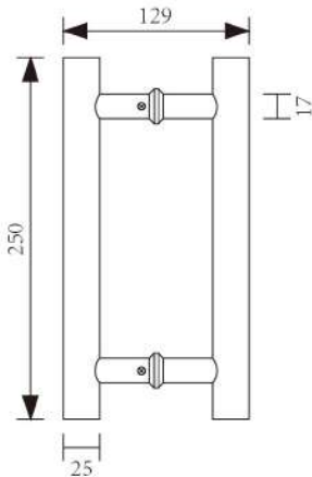
Glass Door Handle MODEL: 102-30mm Material: stainless steel.
