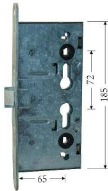
Lc31 Security Lock
