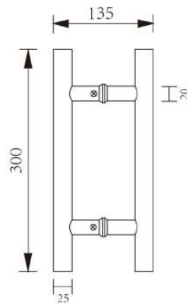
Glass Door Handle Material: stainless steel.
