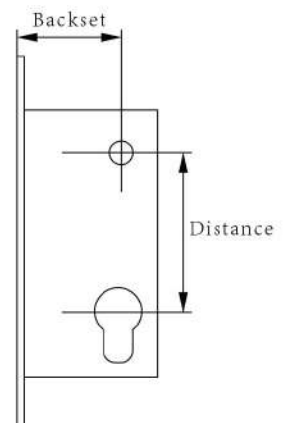
Lc33-5572 Panic Exit Lock
