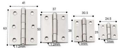
MODEL: SSH024 Stainless Steel Furniture Hinge
