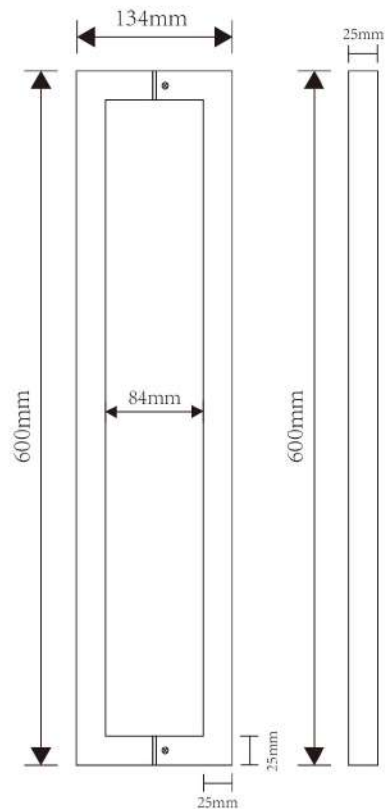
Glass Door Handle Material: stainless steel.
