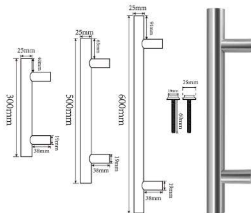
Glass Door Handle
